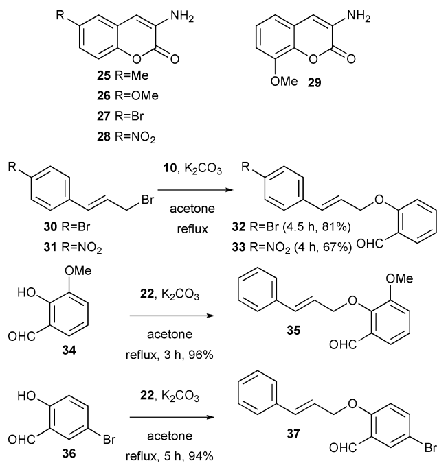
Scheme 7 Synthesis of aldehydes 32 , 33 , 35 and 37 .
